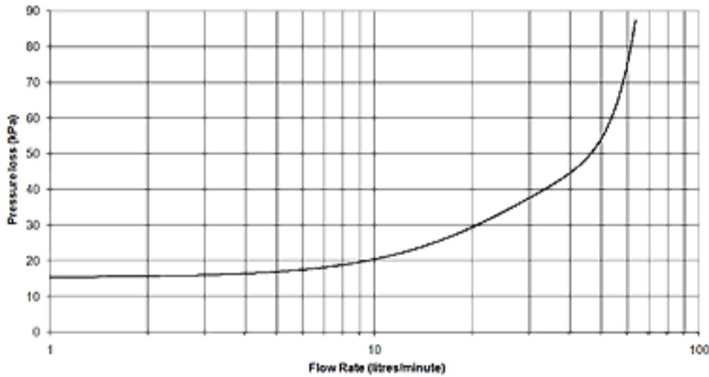
Pressure Loss DW20
