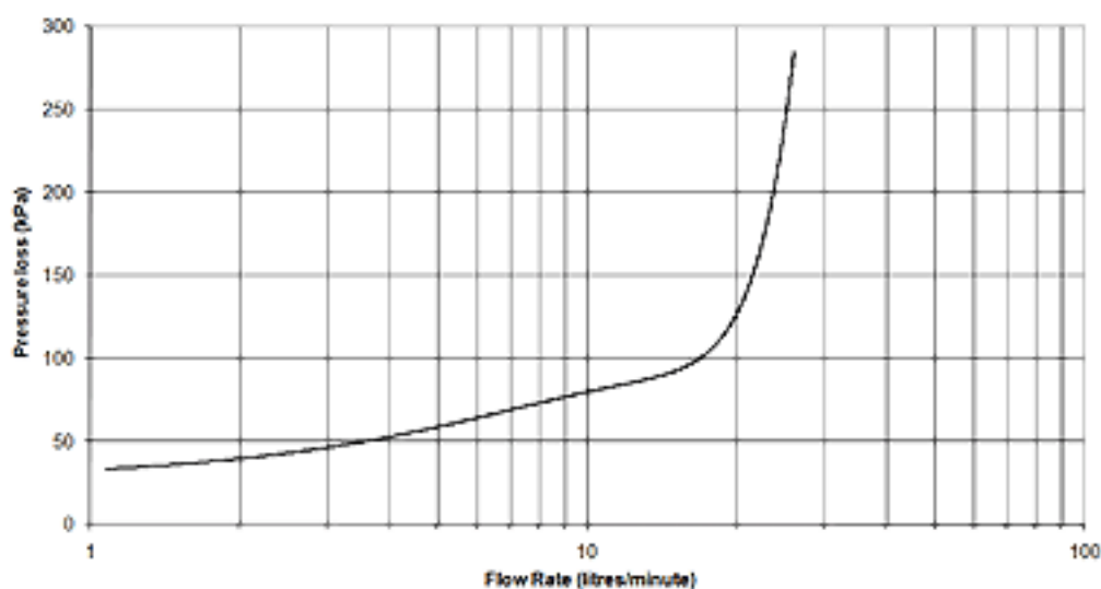
Pressure loss DN14 Dual Check
